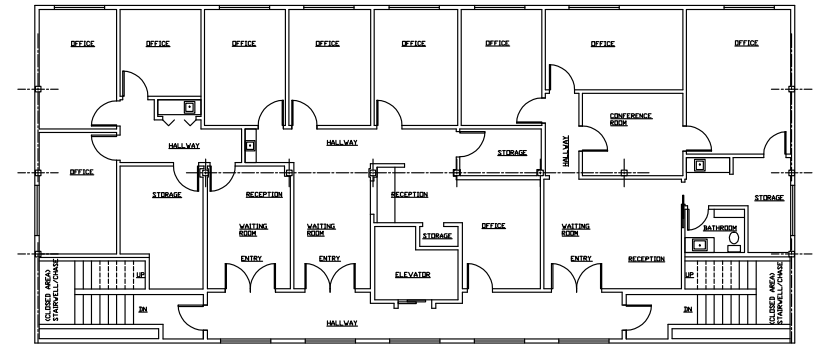
THIRD FLOOR 3660 S.F.
